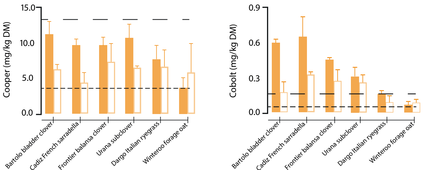
Figure 1. Variation of copper and cobalt in a range of pasture legumes and grass species collected in spring (filled columns) or summer (open columns). Dotted line indicates the bottom of the minimum requirement range for sheep (usually adults at maintenance), dashed line indicates the top of the requirement range (usually growing, pregnant or lactating sheep)?
